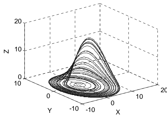
Fig. 8 Constructed Rössler attractor
